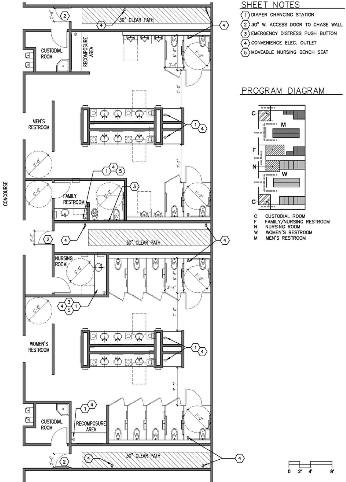
Figure 1.12D RESTROOM CIRCULATION AND FLOOR PLAN PROGRAM
