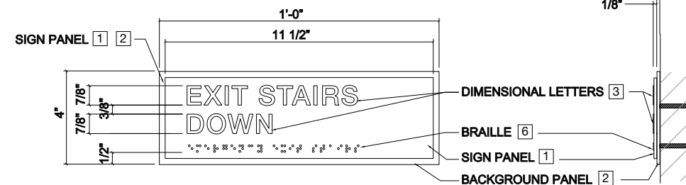
3 FRONT ELEVATION NOT TO SCALE
