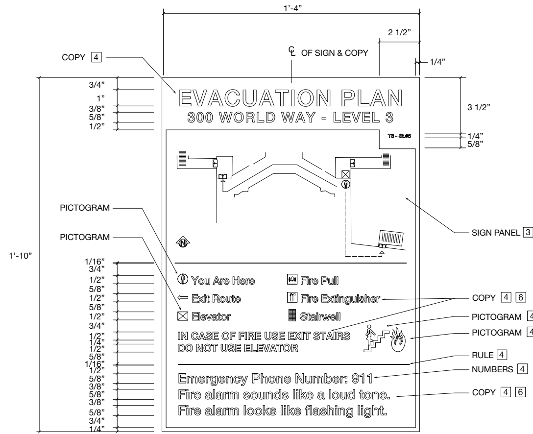
1 FRONT ELEVATION - ALT 1 NOT TO SCALE
