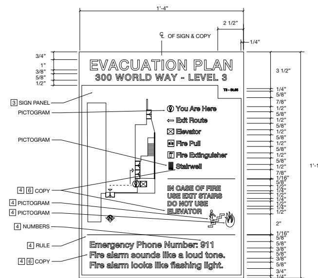
5 FRONT ELEVATION - ALT 2 NOT TO SCALE
