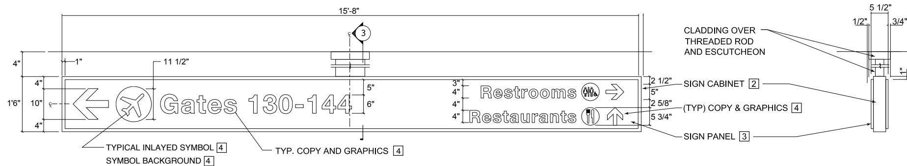
1 FRONT ELEVATION NOT TO SCALE
