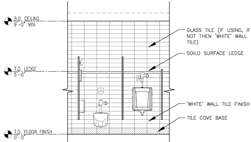
Figure 1.9B5 WALL FINISH AT URINALS AND WATER CLOSETS
