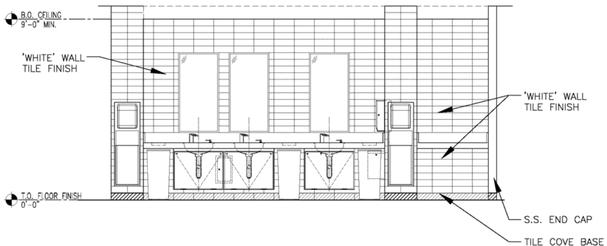
Figure 1.9B3 WALL FINISH AT LAVATORIES
