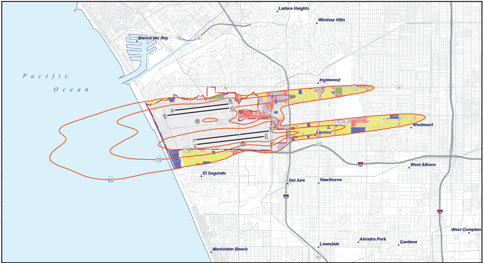
Figure 16 2013 CNEL Contours with Proposed Runway Use Restriction
